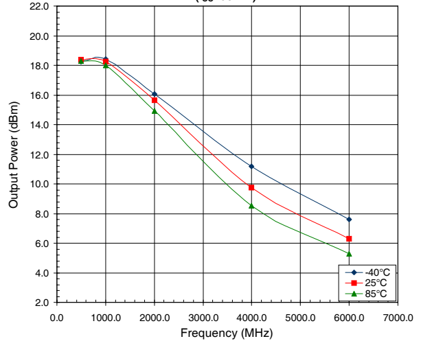
Output P1dB versus Frequency Across Temperature ( I_{CC}=65mA )
